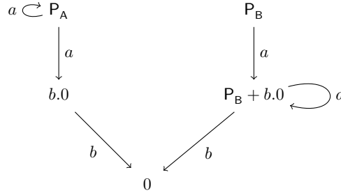
Figure 2: Transition system for P_A and P_B of Example 1, showing only reachable states.
